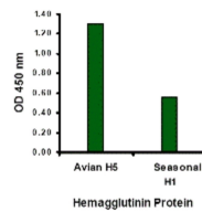
Hemagglutinin antibody at 1 µg/mL specifically recognizes Avian H5N1 influenza virus but not seasonal influenza virus A H1N1 Hemagglutinin protein.
