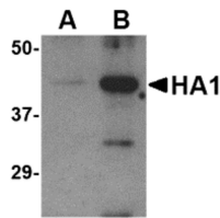
Western blot analysis of (A) 5 ng and (B) 25 ng of recombinant HA1 with Avian Influenza Hemagglutinin antibody at 1 µg/mL.
